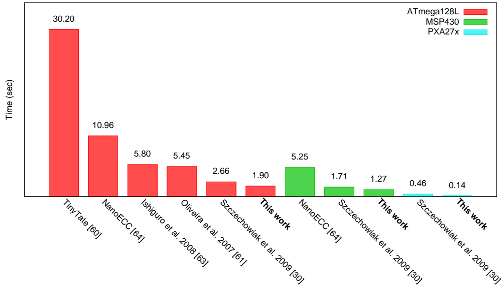
Figure 1. Timings for pairing computation in several sensor platforms.
